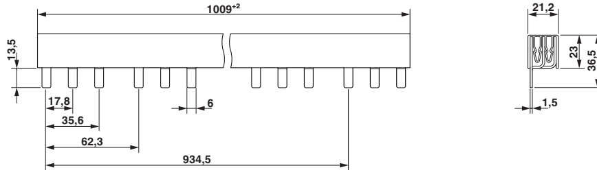
Dimensional drawing
